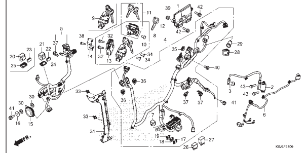
F-41 WIRE HARNESS
